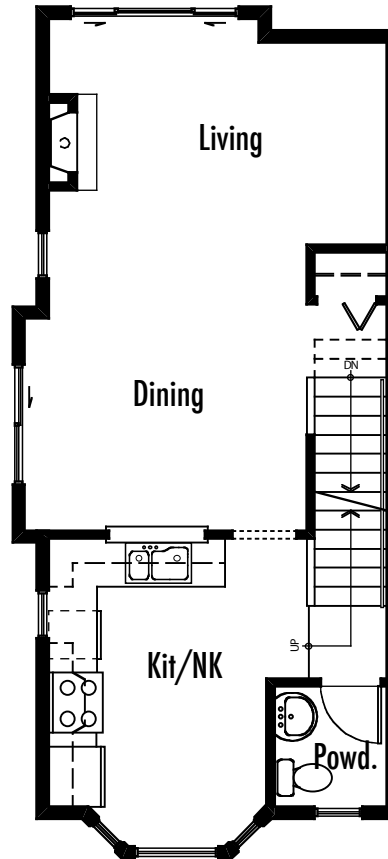
Second Floor 522 SQ.FT.
