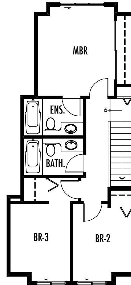
Third Floor 576 SQ.FT.
